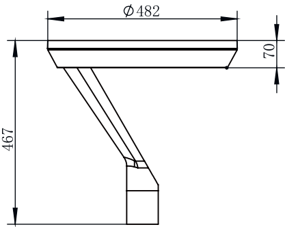
(Fit to D60mm pole)
