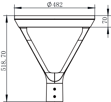
(Fit to D76mm pole)
