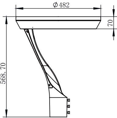
(Fit to D76mm pole)
