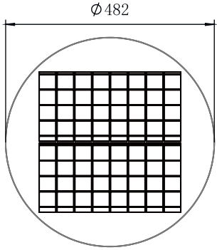
(Fit to D60mm pole)
