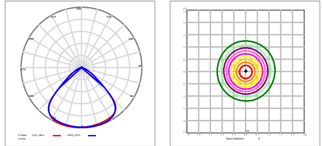
90° Ribbed Lens
